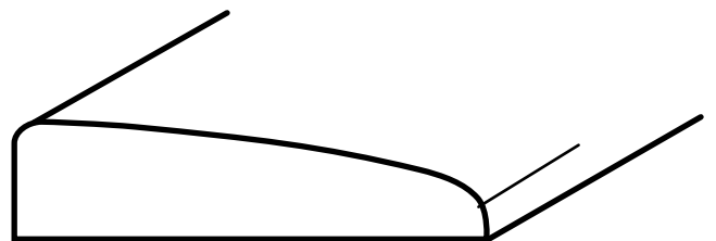
TPI-209 9/16" x 2 1/4"
