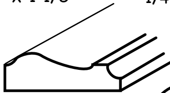
TPI-472 3/8" x 1 3/16"
