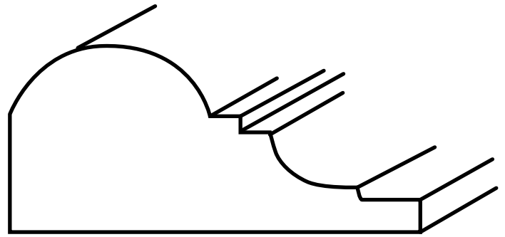
TPI-423 1 3/8" x 3"
