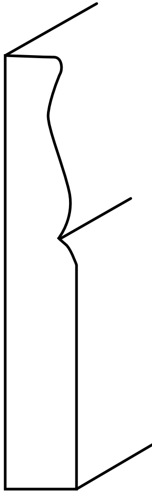
TPI-321 3/4" x 4 1/2"
