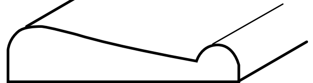
TPI-233 5/8" x 2 3/8"
