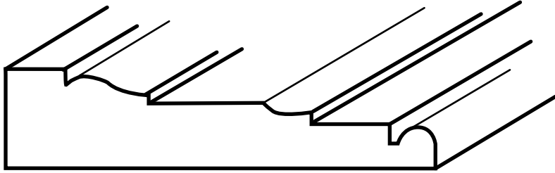
TPI-241 3/4" x 3 1/8"
