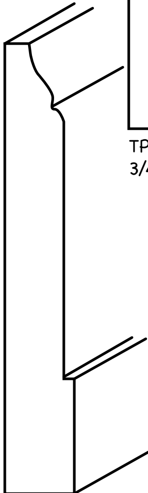
TPI-319 3/4" x 4 3/4"
