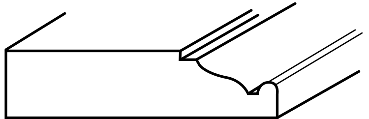
TPI-293 3/4" x 2 3/4"
