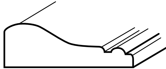
TPI-250 3/4" x 2 1/8"
